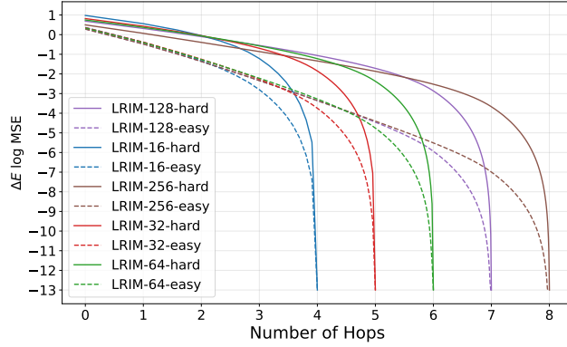
Figure 2: Oracle predictor performance degrades when restricted to consider local r -hop neighborhoods only. The oracle uses the true underlying energy function, but only considers spins within hop-distance r from each target node. Results demonstrate that smaller \sigma values (harder tasks) require larger neighborhoods to achieve the same accuracy, confirming stronger long-range dependencies. Second, larger system sizes increase task difficulty, even within the same \sigma . Moreover, the performance decays smoothly, providing a continuous feedback both during evaluation and training. Therefore, achieving low prediction error requires information from neighborhoods spanning significant fractions of the graph, providing model-agnostic evidence that local information is insufficient.
