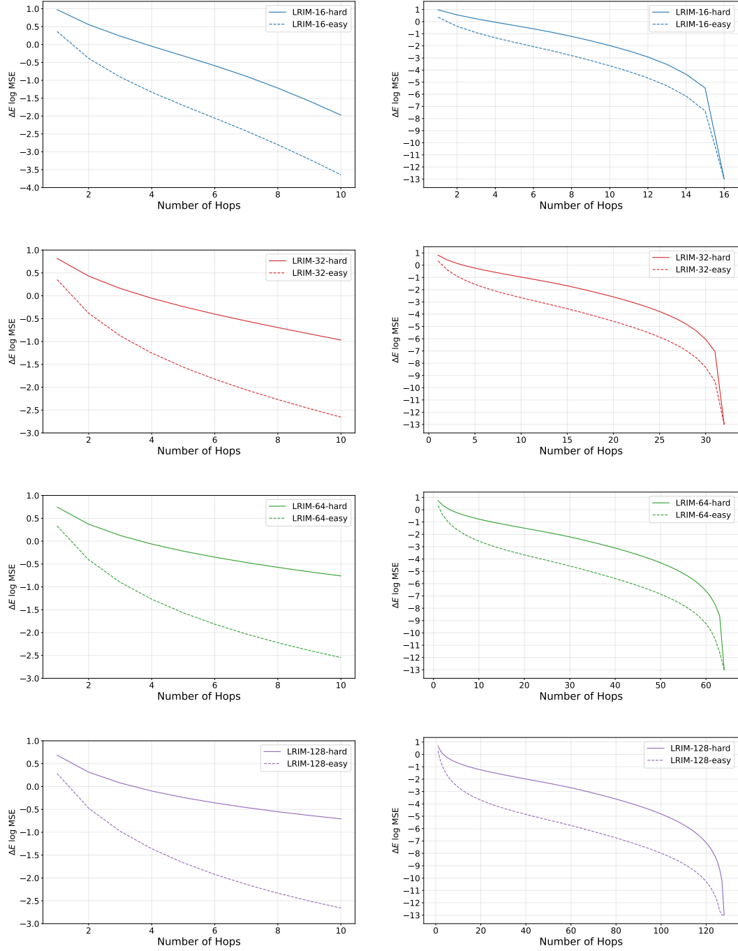
Figure 7: Oracle predictor performance across a single LRIM dataset when restricted to r -hop neighborhoods. (Left) indicates the first 10 hops, while (right) shows performance across the graph diameter. Performance degrades smoothly as neighborhood size decreases. Further, harder variants consistently require larger neighborhoods than easier variants for the same accuracy. Finally, larger sizes also increase task difficulty even for fixed \sigma . The oracle uses the true underlying Ising energy function but only considers spins within hop-distance r , providing model-agnostic evidence that our benchmark tasks genuinely require long-range information across substantial parts of the graph.
