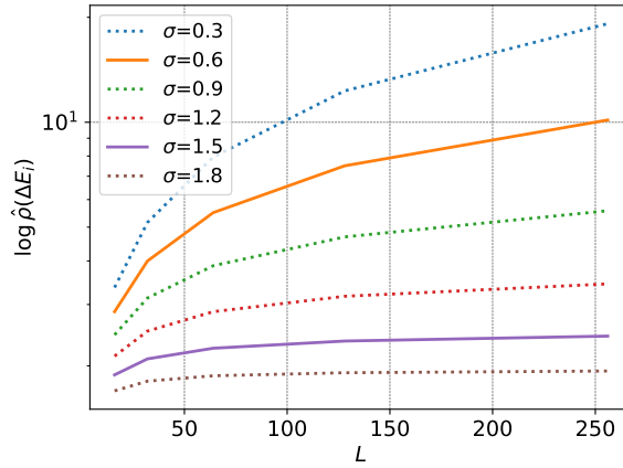
Figure 15: Normalized node range for the graph shortest path distance metric with different sigma. The experiments are run over Ising models with even grid size. \sigma for Ising models for solid lines is identical to that reported in Table 1. The dotted lines correspond to additional \sigma introduced to visualize trend in the long-range metric when varying \sigma .
