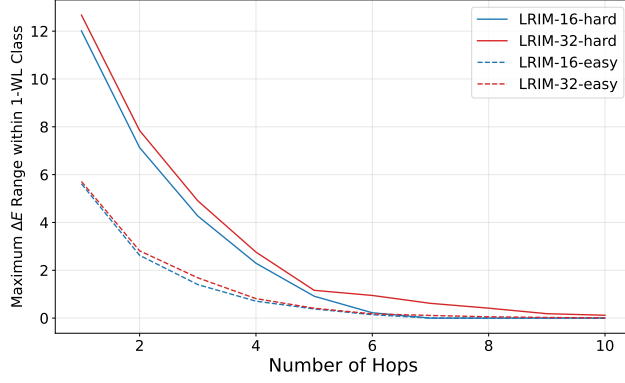
Figure 11: Maximum range of \Delta E values among nodes sharing the same 1-WL equivalence class when restricted to r -hop neighborhoods. Nodes that are indistinguishable to message-passing neural networks can initially exhibit vastly different energy targets, requiring expanded receptive fields to resolve these ambiguities. However, they decay much faster than the oracle predictor (Figure 2) indicates potential overfitting with finite data, though generalization likely requires distances closer to the oracle. However, this also means that inherently, 1-WL in distinguishability should not pose a major obstacle for MPNNs on our Benchmark.
