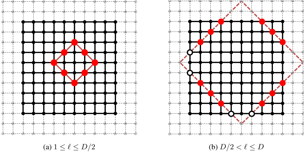
Figure 14: Visualization of contributing spins on H with size (L+1) \times (L+1) for L = 9 (= D+1) , depending on graph shortest path distance d_G(i, k) = \ell . Dotted circles are complementary virtual spins located outside of H which is drawn by solid lines and circles. Red solid lines represent x \pm y = \pm \ell and red solid circles are spins composing N_\ell(i) .
