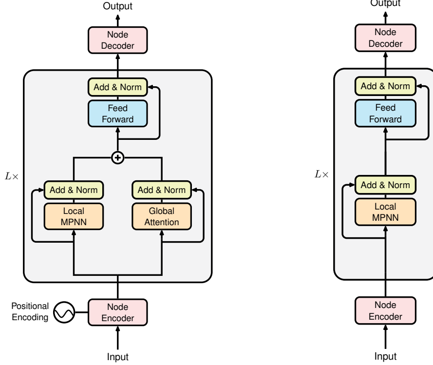
Figure 12: Baseline model architectures used in our evaluation. (Left) Graph transformer (GPS) combines local message-passing with global attention, allowing nodes to directly attend to all other nodes in the graph. (Right) Message-passing neural network (MPNN) rely on local neighborhood aggregation through multiple layers to expand the receptive field. Both architectures use the identical overarching block structure including normalization, skip-connections and Feed Forward Networks stacked L times. Figure design is inspired by the overview of Vaswani et al. (2017).
