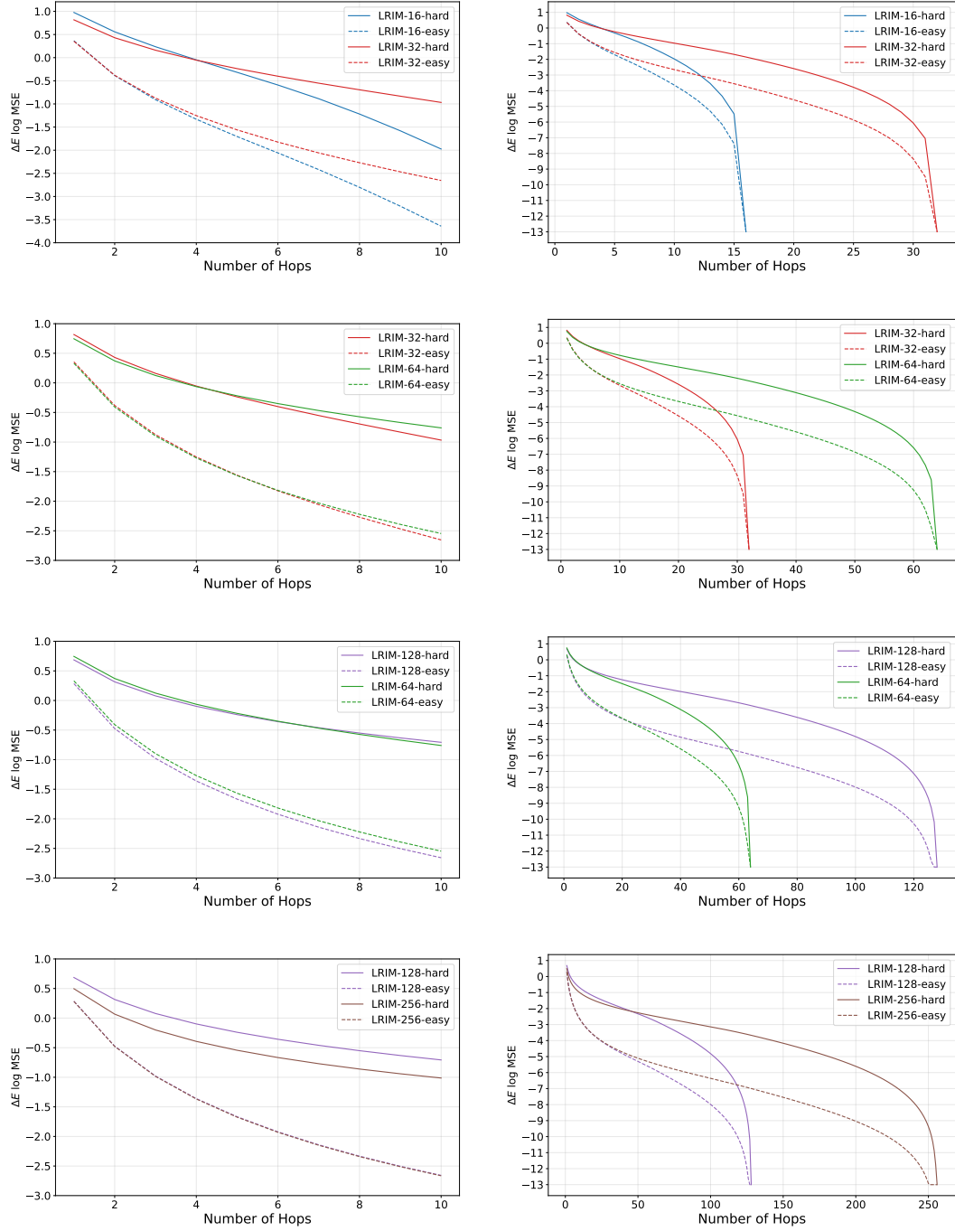
Figure 6: Oracle predictor performance across size adjacent LRIM datasets when restricted to r -hop neighborhoods. (Left) indicates the first 10 hops, while (right) shows performance across the graph diameter. Performance degrades smoothly as neighborhood size decreases. Further, harder variants consistently require larger neighborhoods than easier variants for the same accuracy. Finally, larger sizes also increase task difficulty even for fixed \sigma . The oracle uses the true underlying Ising energy function but only considers spins within hop-distance r , providing model-agnostic evidence that our benchmark tasks genuinely require long-range information across substantial parts of the graph.
