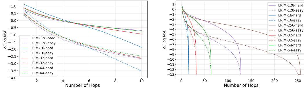
Figure 5: Oracle predictor performance across all LRIM datasets when restricted to r -hop neighborhoods. (Left) indicates the first 10 hops, while (right) shows performance across the graph diameter. Performance degrades smoothly as neighborhood size decreases. Further, harder variants consistently require larger neighborhoods than easier variants for the same accuracy. Finally, larger sizes also increase task difficulty even for fixed \sigma . The oracle uses the true underlying Ising energy function but only considers spins within hop-distance r , providing model-agnostic evidence that our benchmark tasks genuinely require long-range information across substantial parts of the graph.
